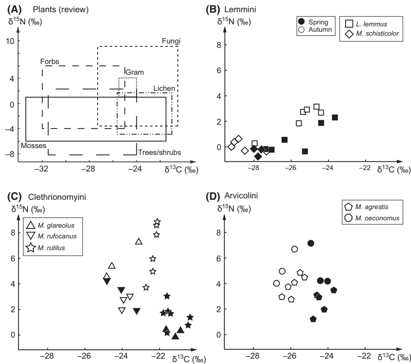
Figure 1. (A) Review of carbon ( \delta^{13}\text{C} ) and nitrogen ( \delta^{15}\text{N} ) isotopic compositions (in ‰) of plant types. The ranges for mosses are based on Nadelhoffer et al. (1996), Brooks et al. (1997), McLeman (2006), and Loisel et al. (2009). Ranges for other plant types are summarized from Ben-David et al. (2001) and Drucker et al. (2010, 2012). gram = graminoids. (B–D) Carbon and nitrogen isotopic compositions of the teeth studied. Black symbols for specimens trapped in spring; white symbols for autumn. (B) Lemmini: Lemmus lemmus (squares) and Myopus schisticolor (diamonds). (C) Clethrionomyini: Myodes glareolus (upright triangles), M. rufocanus (inverted triangles) and M. rutilus (stars). (D) Arvicolini: Microtus agrestis (pentagons) and M. oeconomus (octagons). Note that (A) and (B–D) are not drawn in the same isotopic space.
